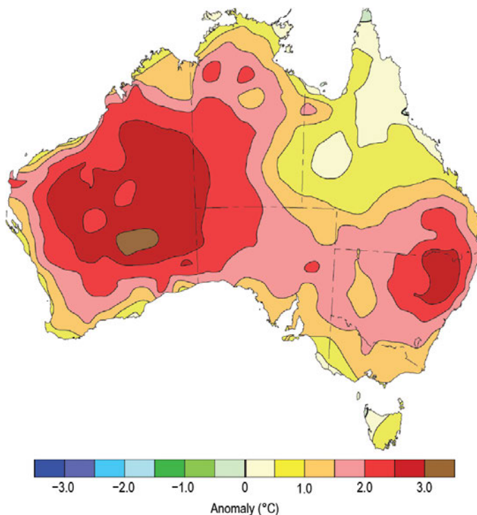
Fig. 7.54. Maximum temperature anomalies ( ^\circ\text{C} ) for Australia, averaged over 2019, relative to a 1981–2010 base period. (Source: Australian Bureau of Meteorology.)
