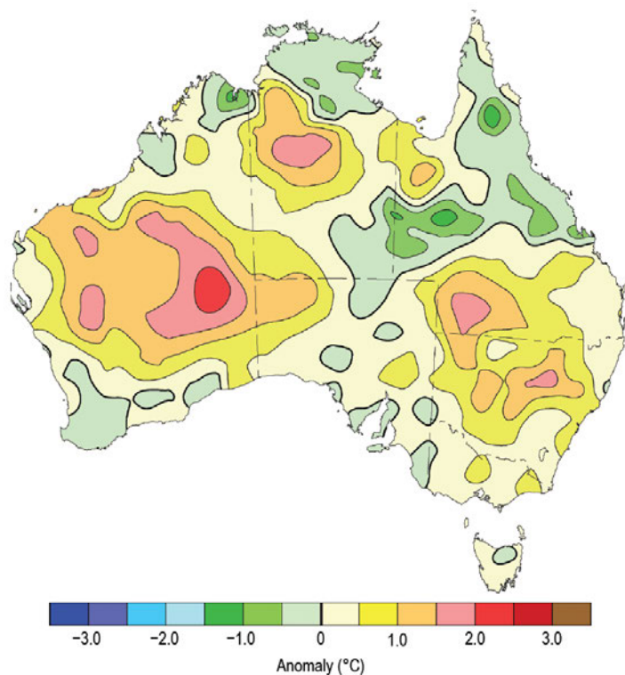
Fig. 7.55. Minimum temperature anomalies (°C) for Australia, averaged over 2019, relative to a 1981–2010 base period. (Source: Australian Bureau of Meteorology.)
