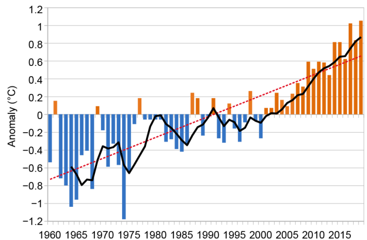
Fig. 7.28. Annual mean temperature anomalies (°C; 1981–2010 base period) in Mauritius, 1960–2019. Black line is the 5-year running mean. The linear trend for the period of record is shown as a dashed line. (Source: Mauritius Meteorological Service.)
