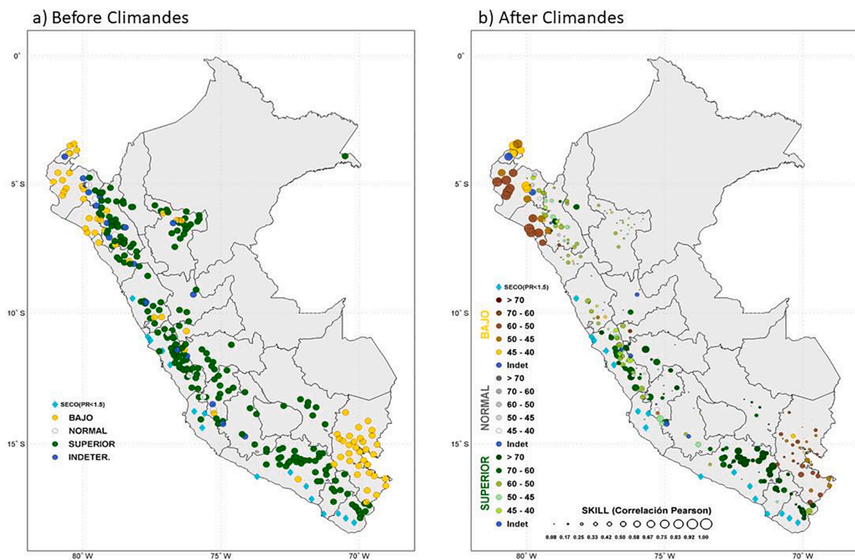
Fig. 6. SENAMHI’s seasonal forecast product before (left) and after (right) Climandes. While the product before Climandes appears as a deterministic true forecast, the seasonal forecasts after Climandes include information on skill and uncertainty.
